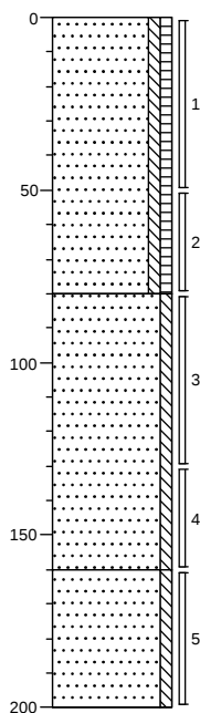
Boring: 01
