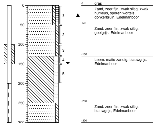
Boring: 2
