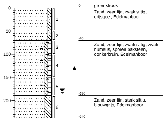
Boring: 3
