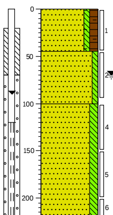
Boring: 16
