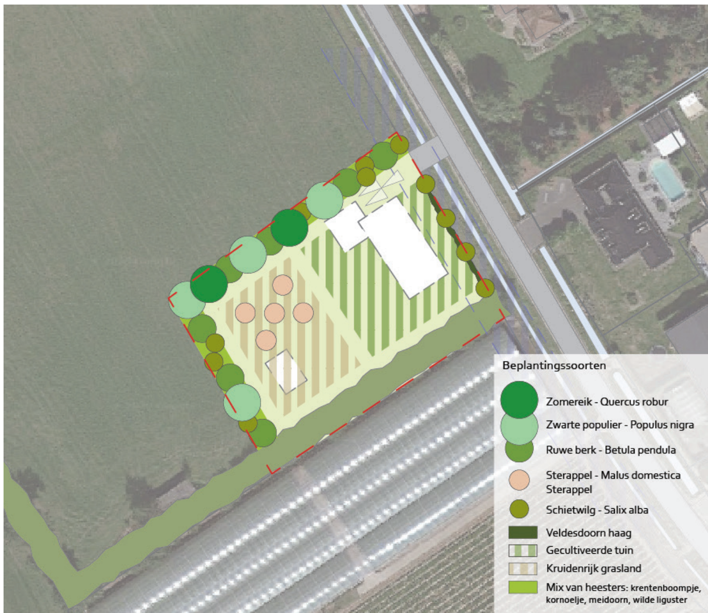
Beplantingsplan
