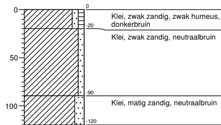
Boring 424
