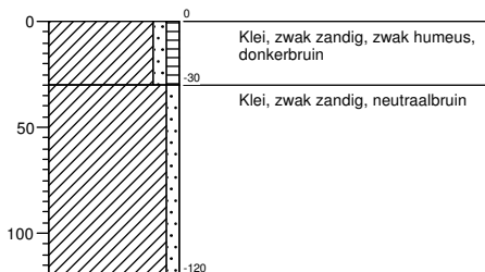
Boring 395
