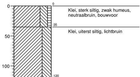
Boring 287
