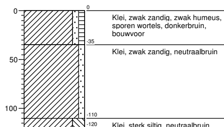
Boring 157
