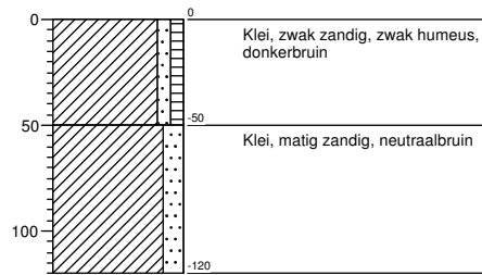
Boring 421
