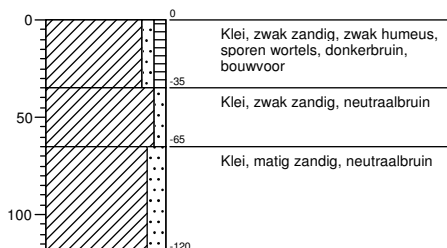
Boring 065
