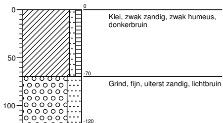
Boring 280
