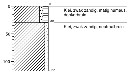
Boring 366
