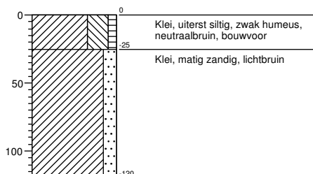
Boring 418
