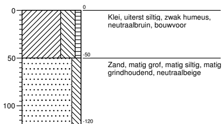
Boring 262
