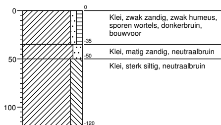
Boring 159
