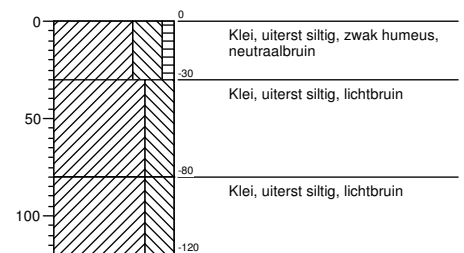
Boring 432
