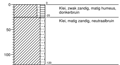
Boring 422
