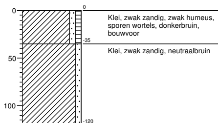
Boring 153
