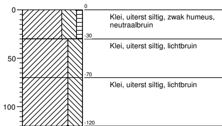
Boring 426
