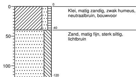
Boring 150
