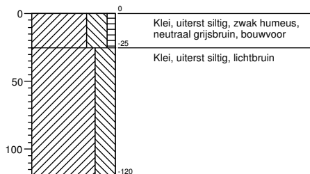
Boring 229
