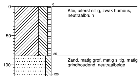
Boring 264
