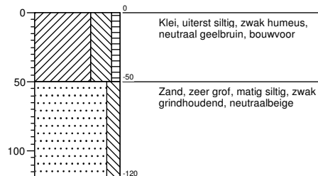
Boring 275
