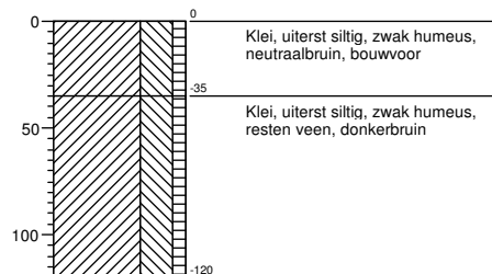
Boring 291
