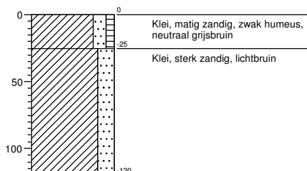
Boring 468
