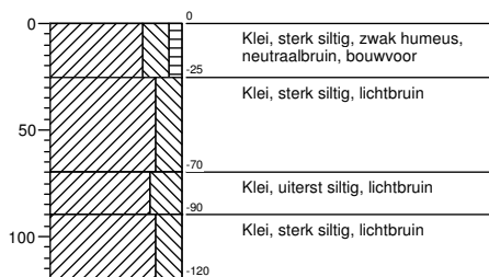
Boring 149
