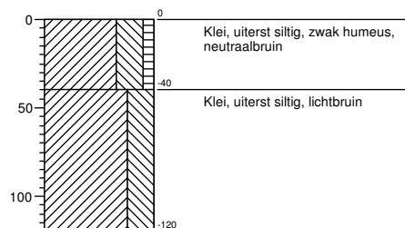
Boring 256
