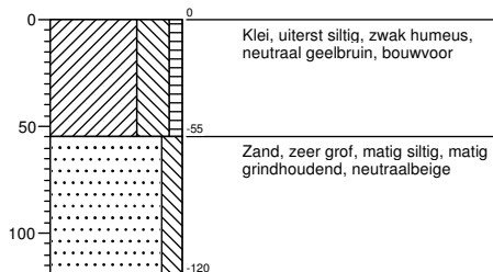
Boring 273
