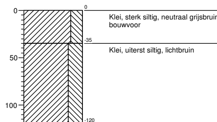
Boring 118
