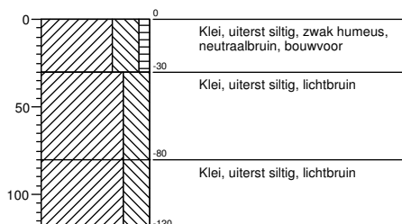
Boring 267
