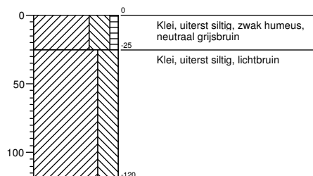
Boring 170
