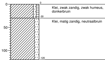
Boring 420
