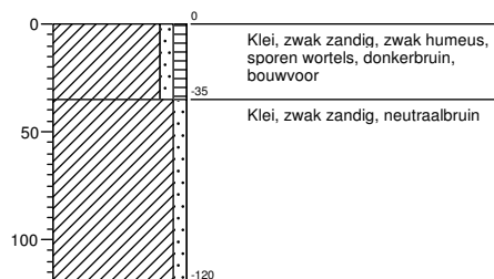
Boring 154
