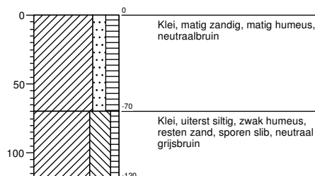
Boring 470
