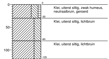
Boring 425
