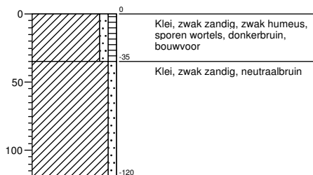
Boring 146
