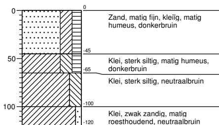
Boring 430
