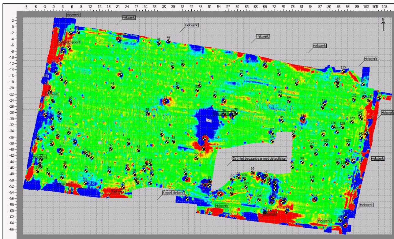
Veld-001, 10nT
