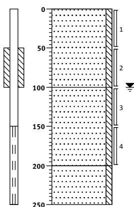
Boring: 710
