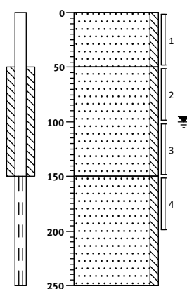
Boring: 711
