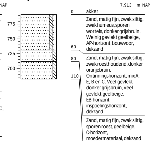
Boring: 4
