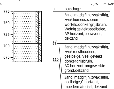
Boring: 2
