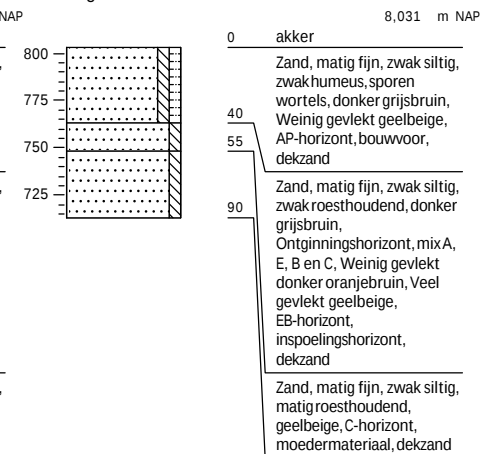
Boring: 8
