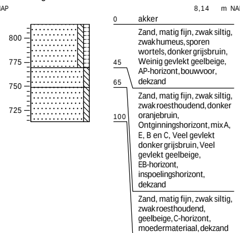
Boring: 7
