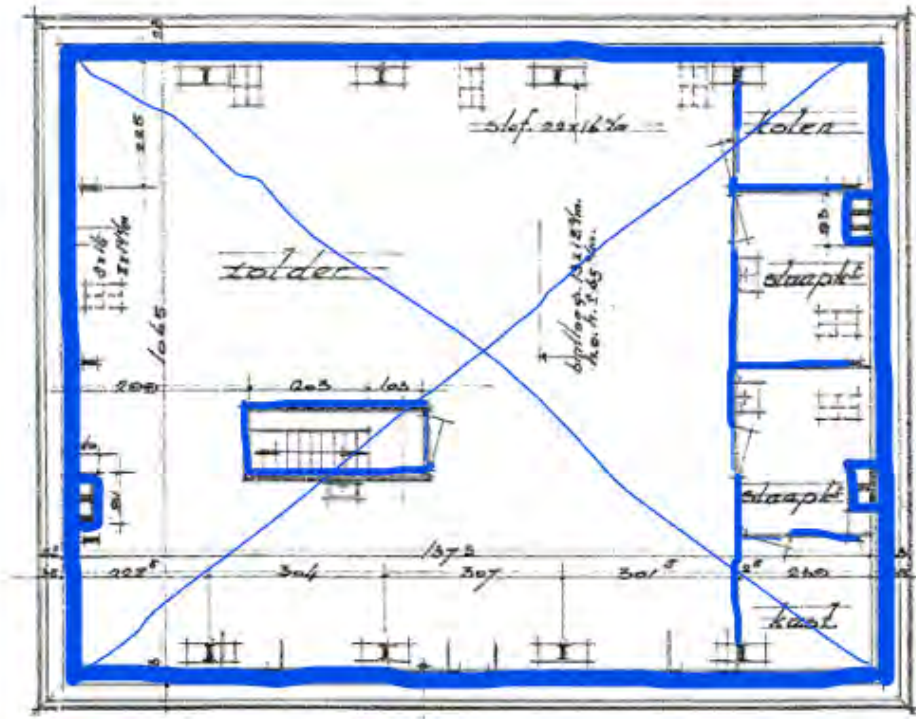
ZOLDERVERDIEPING
