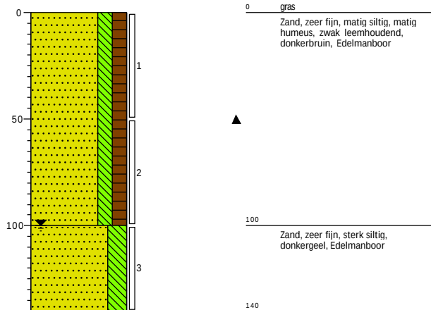
Boring: 01
