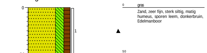
Boring: 04
