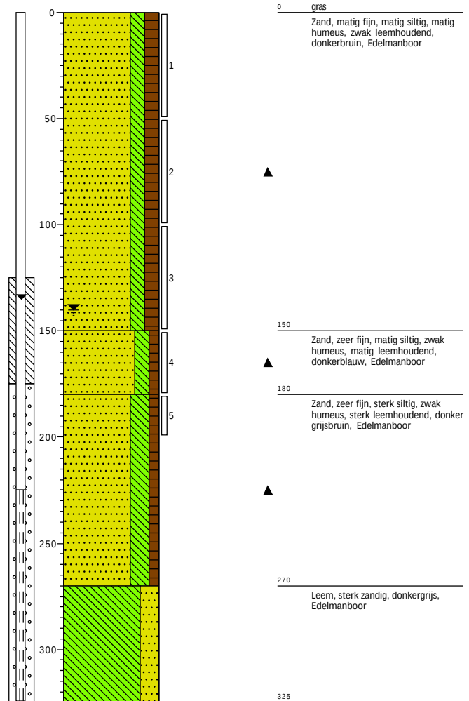
Boring: 02
