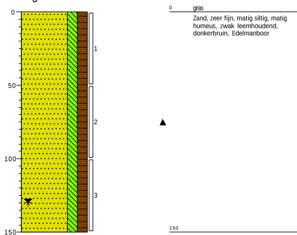
Boring: 03
