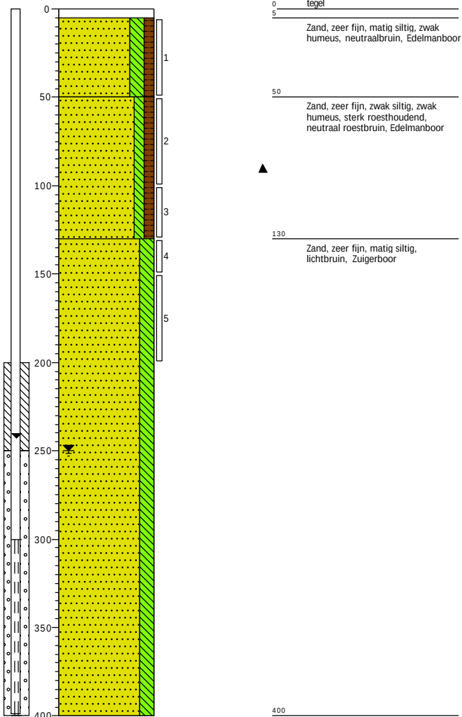
Boring: 01
