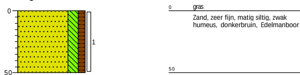
Boring: 03
