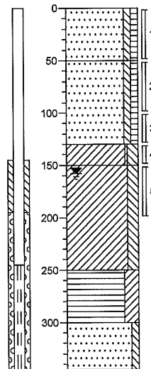
Boring: 02
