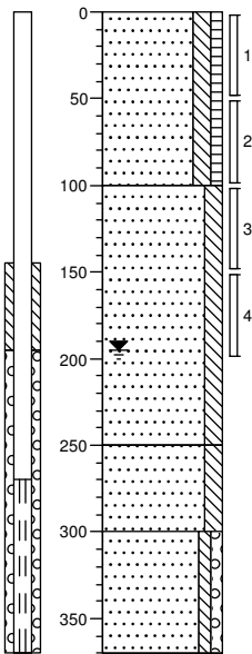
Boring: 08
