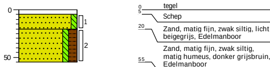
Boring: 10
