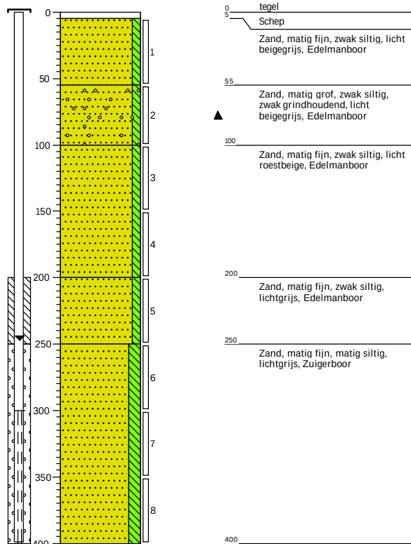
Boring: 07
