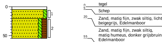
Boring: 04
