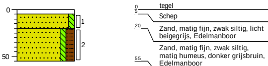
Boring: 09
