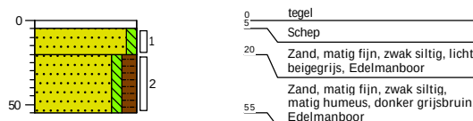
Boring: 06
