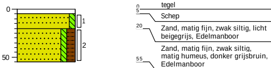
Boring: 11
