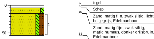
Boring: 12
