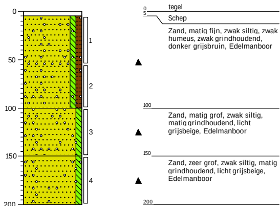
Boring: 03
