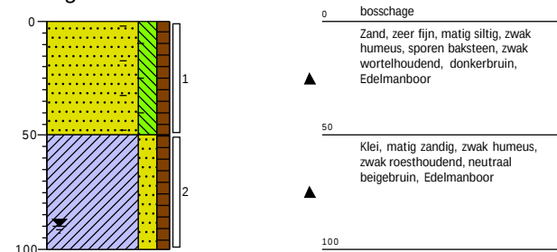
Boring: 02
