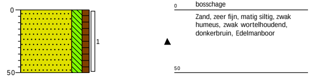
Boring: 14
