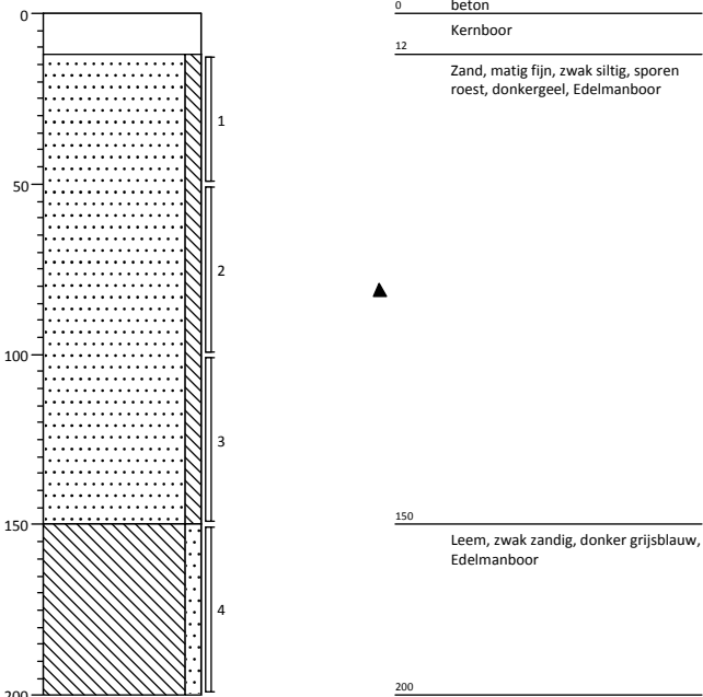
Boring: 02
