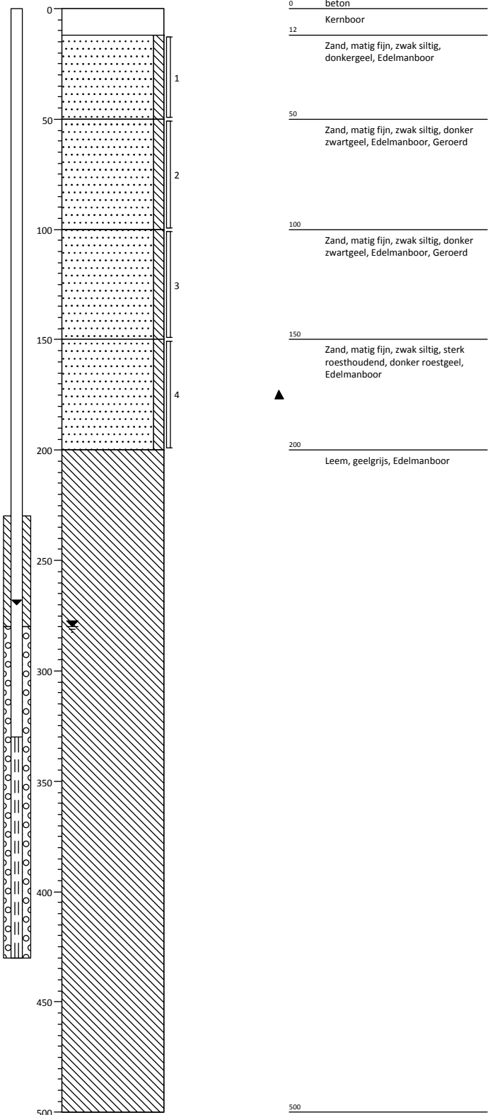
Boring: 01
