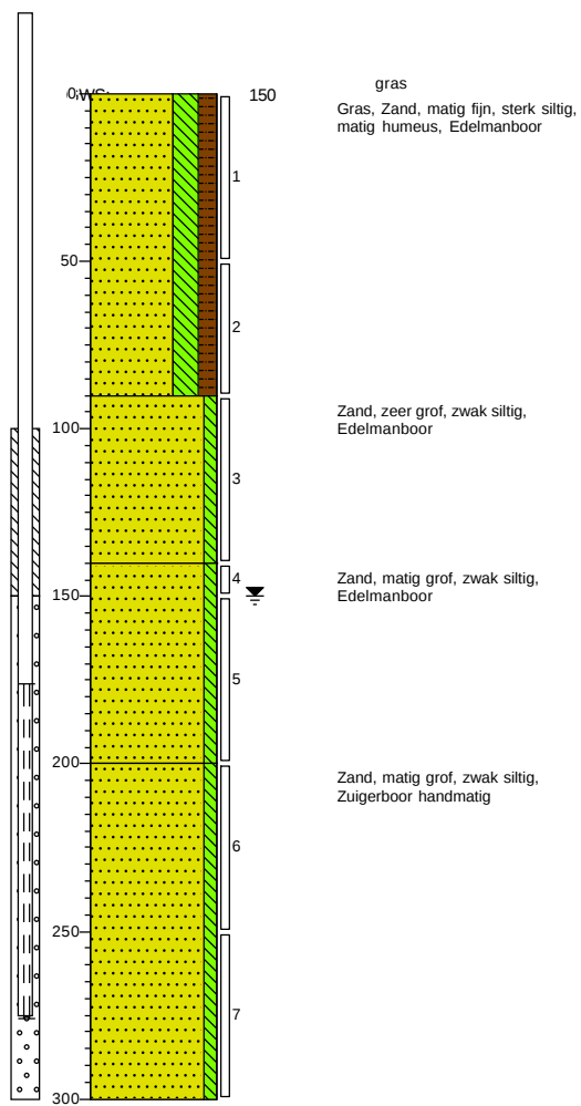
Boring: 23
