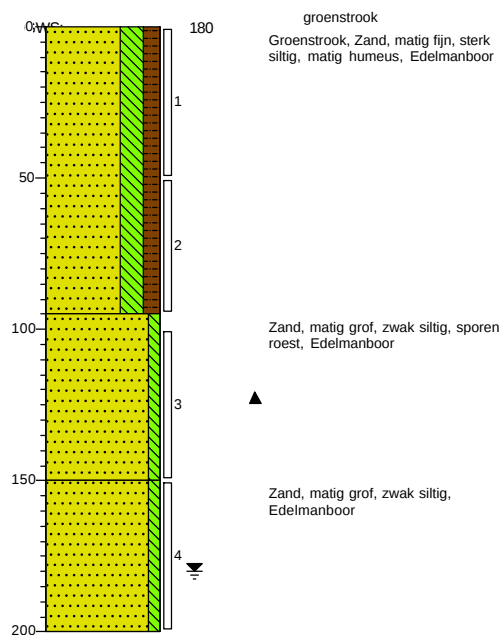
Boring: 14
