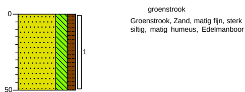
Boring: 16
