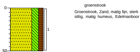
Boring: 15
