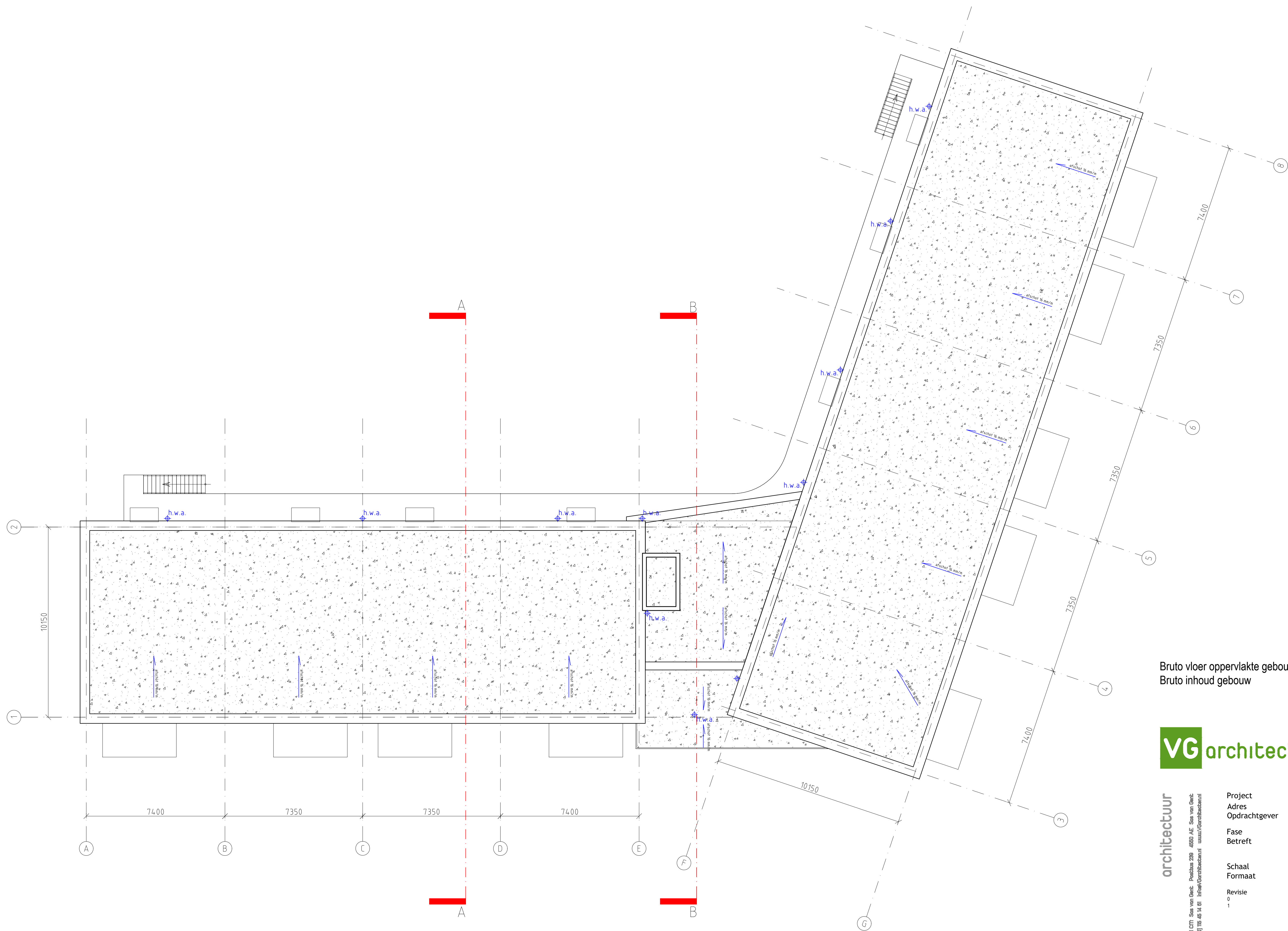
DAKPLAN
