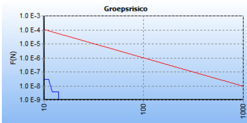
Figuur 5.12 FN-curve W-528-03
