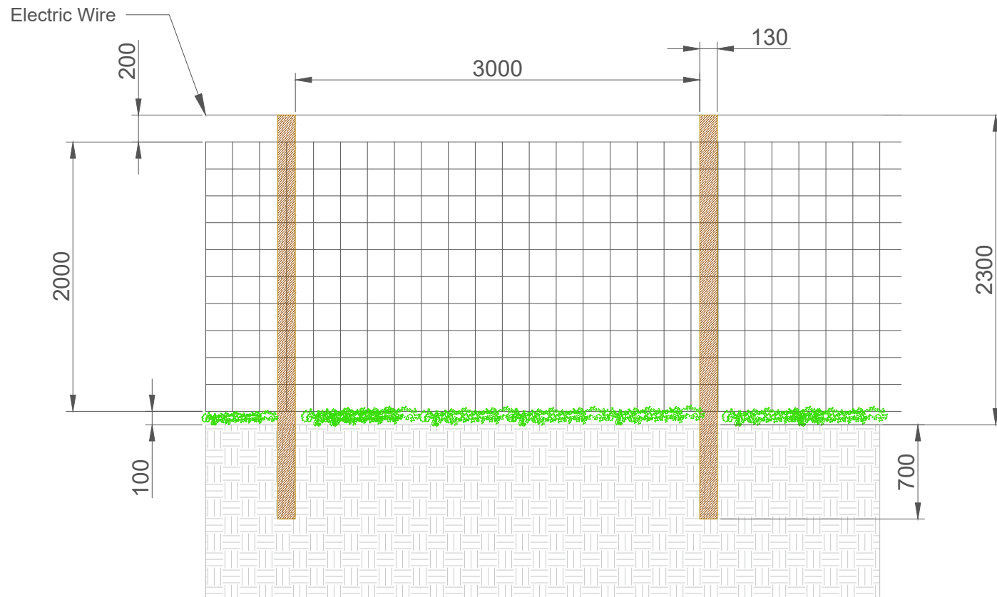
Illustration Eco-Friendly Fence
