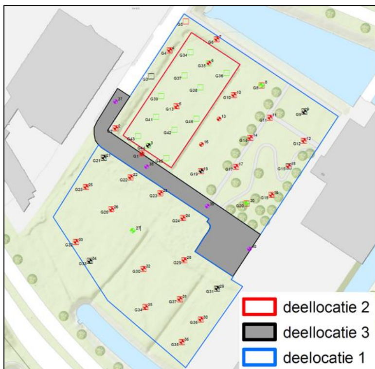
Boorplan (bron: ATKb 2019)
