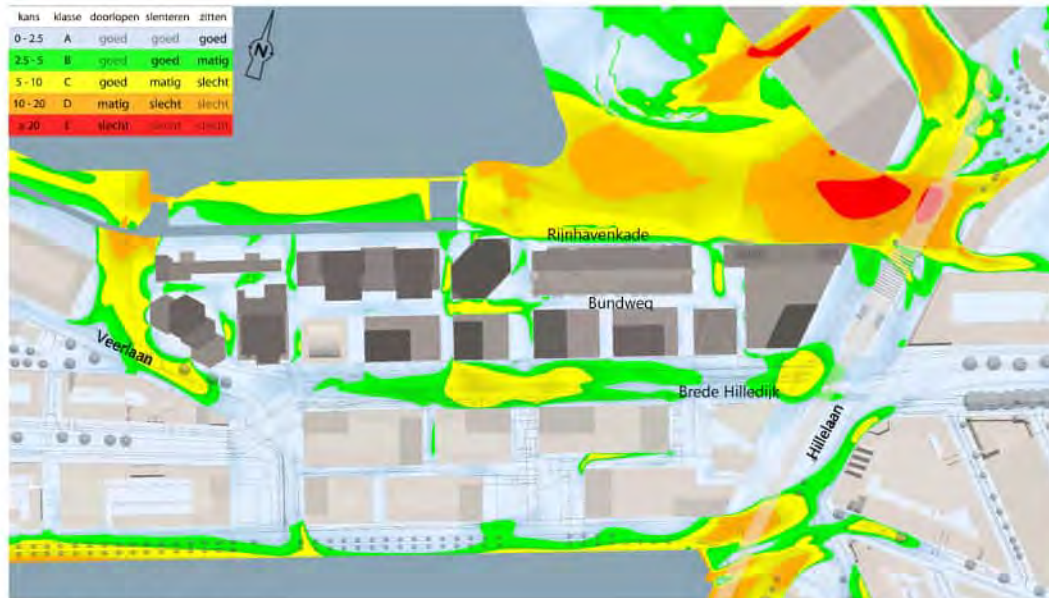
f 3.5 Windhinder in de plansituatie
