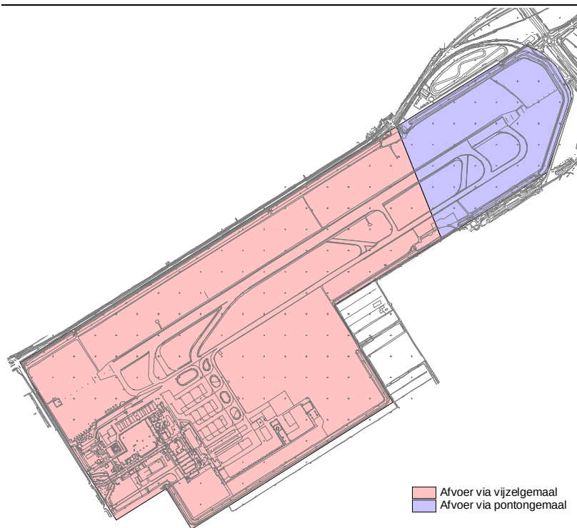
Figuur 4.3 Afwatering Rotterdam The Hague Airport
