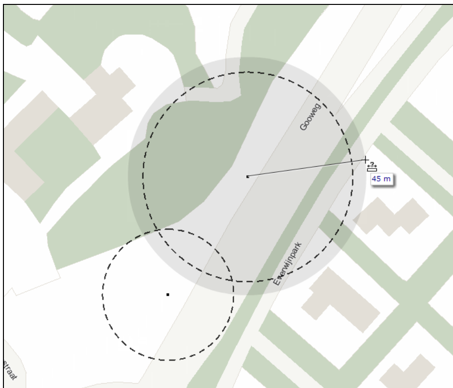
Figuur 6: PR=10^{-6} contour vulpunt LPG-tankstation Texaco Abswoude
