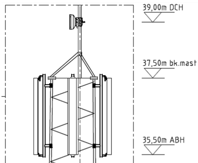
Placement of the antennas
