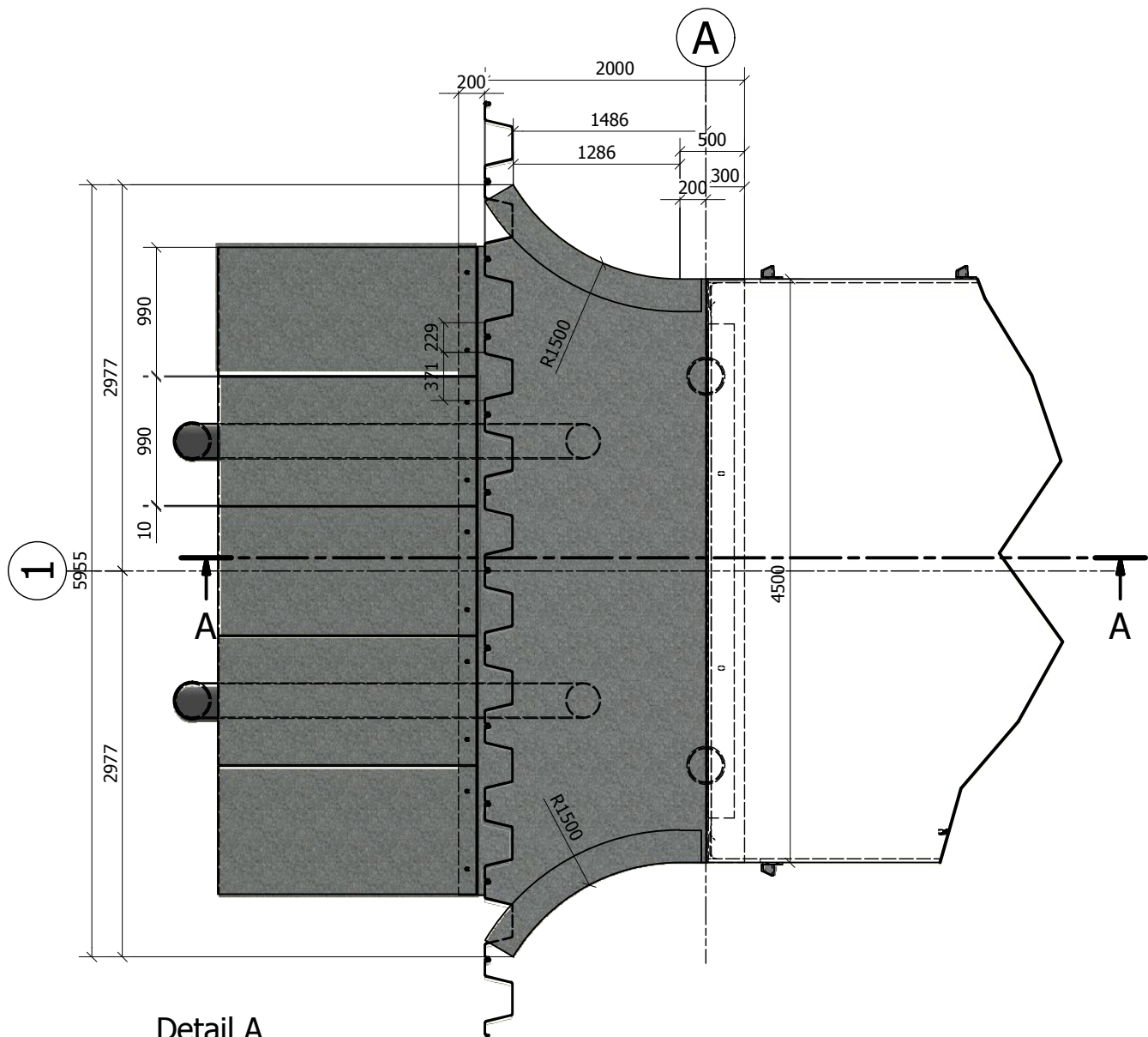
Detail A
