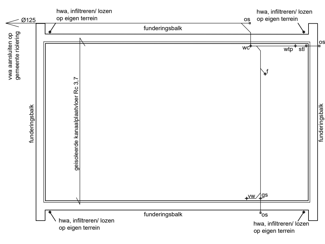
principe fundering/ riolering/ begane grondvloer
