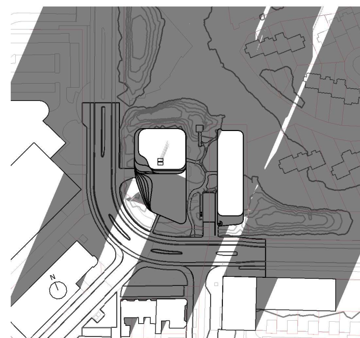
21 december 16:00 1 : 2000
