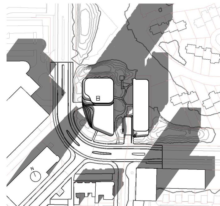
21 september 16:00 1 : 2000
