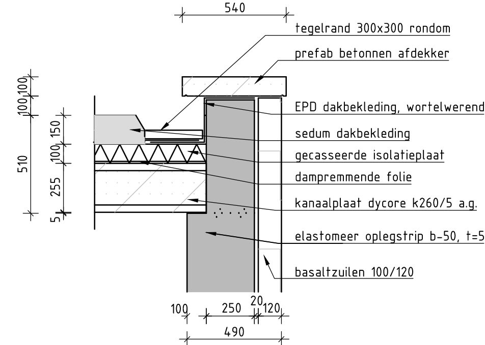
DETAIL 1: OPLEGGING schaal 1:20
