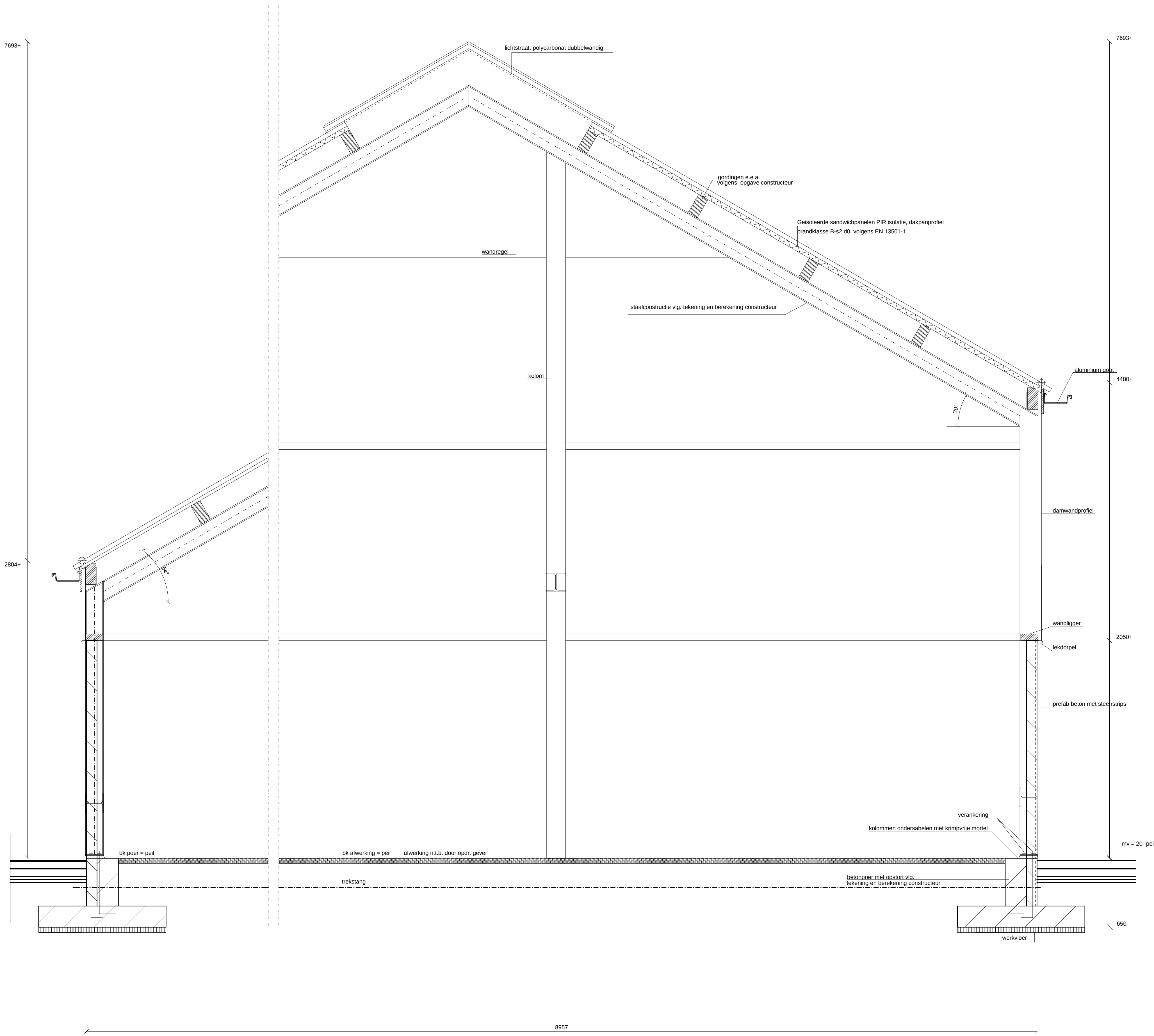
details a-a
