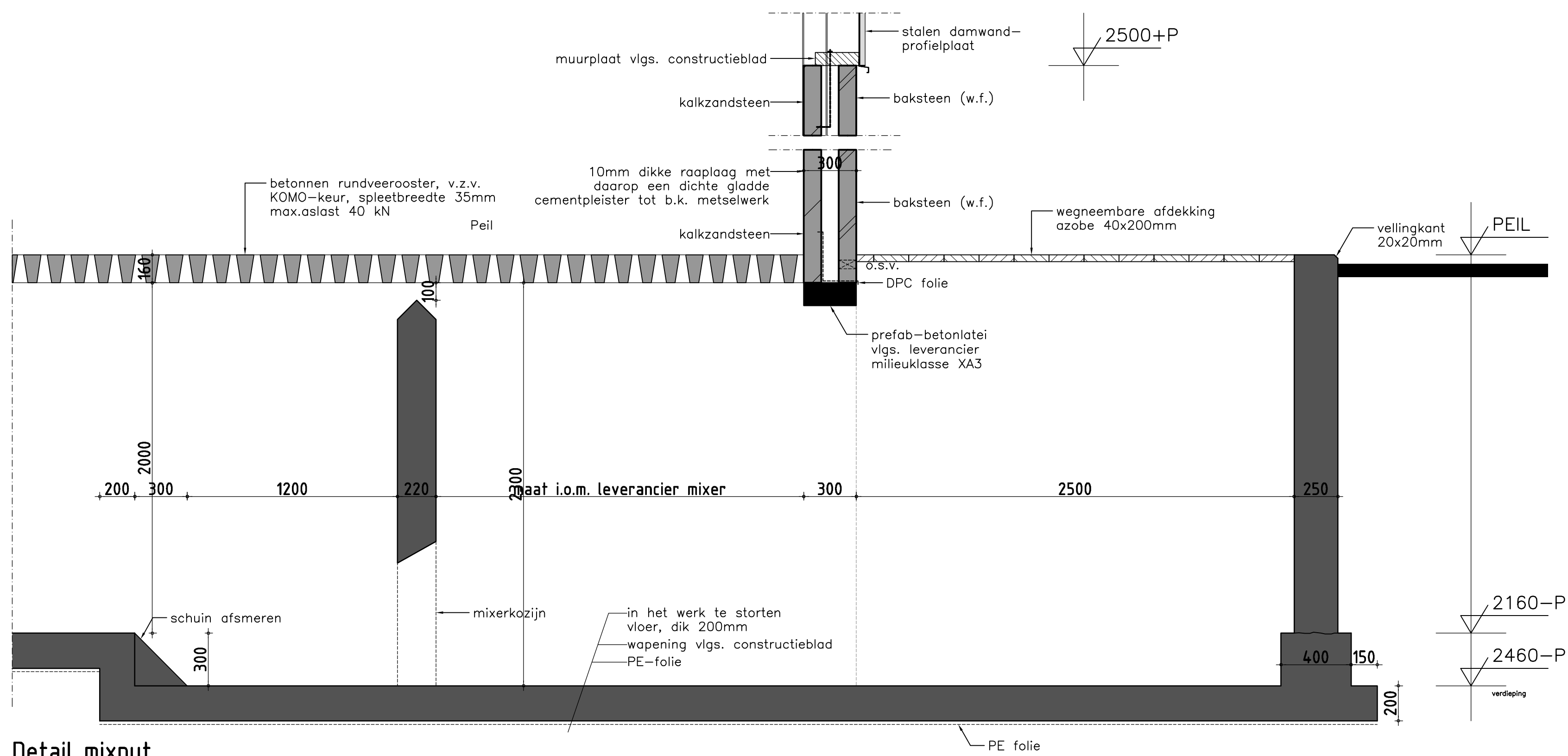
Detail mixput
