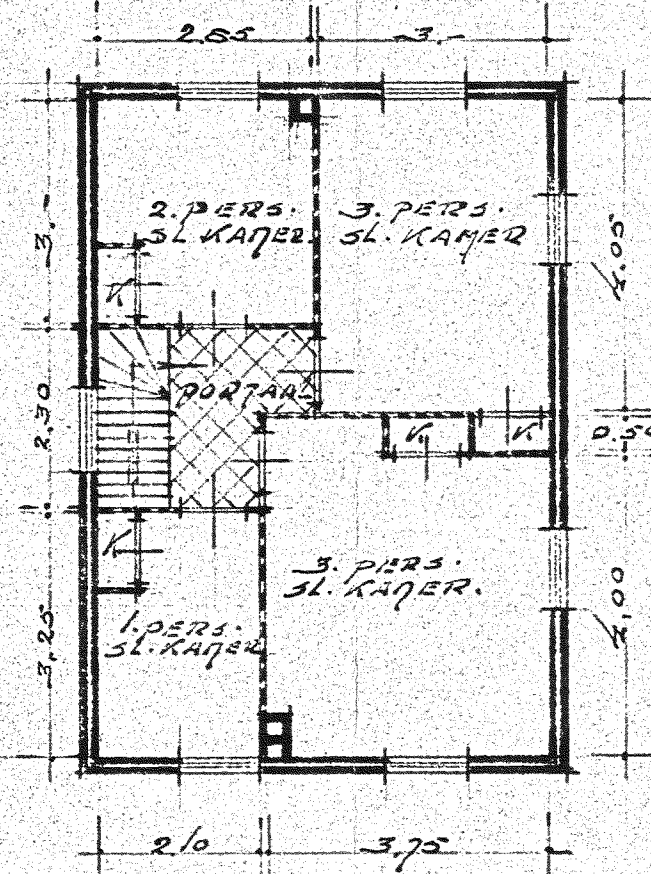
VERDIKPING.
