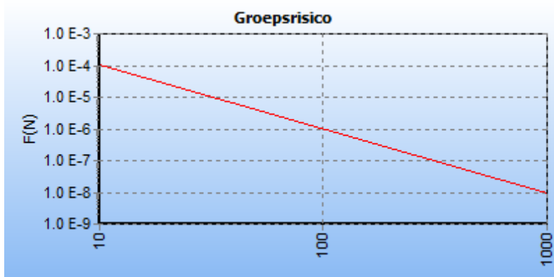
Figuur 2.1 FN-Curve
