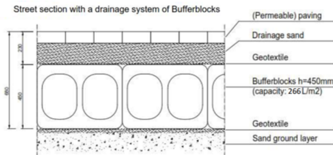
Figuur 6-6 Principe Bufferblocks (Bron: Bufferblock product information, Bufferblock, 2024).
