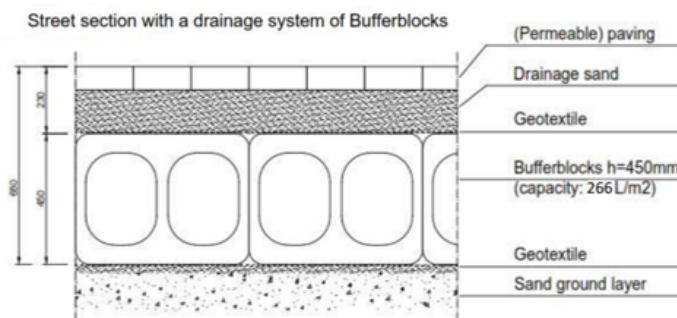
Figuur 7-5 Principe Bufferblocks (Bron: Bufferblock product information, Bufferblock, 2024).
