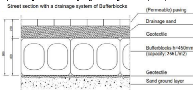
Figuur 5-6 Principe Bufferblocks (Bron: Bufferblock product information, Bufferblock, 2024).
