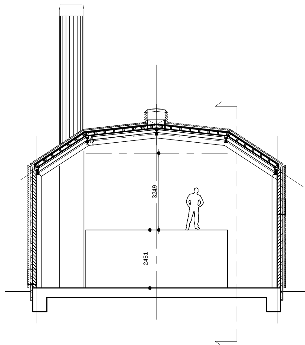
dwarsdoorsnede as 4
