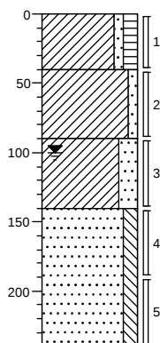
Boring: 01
