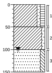
Boring: 02
