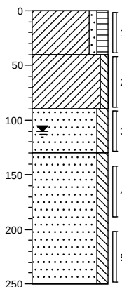
Boring: 16
