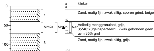
Boring: 13
