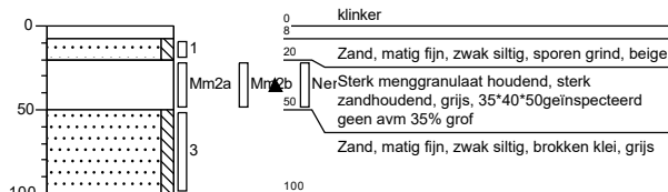
Boring: 11
