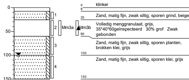
Boring: 14
