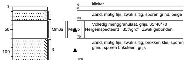
Boring: 15
