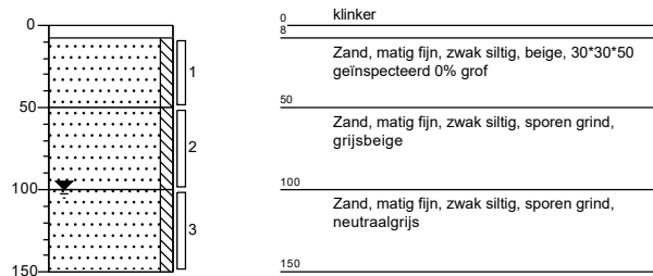
Boring: 12
