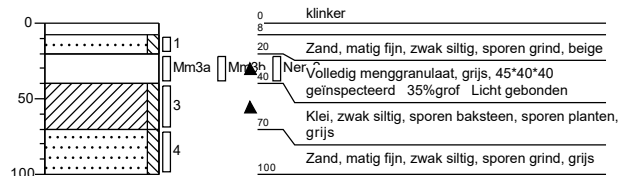
Boring: 16
