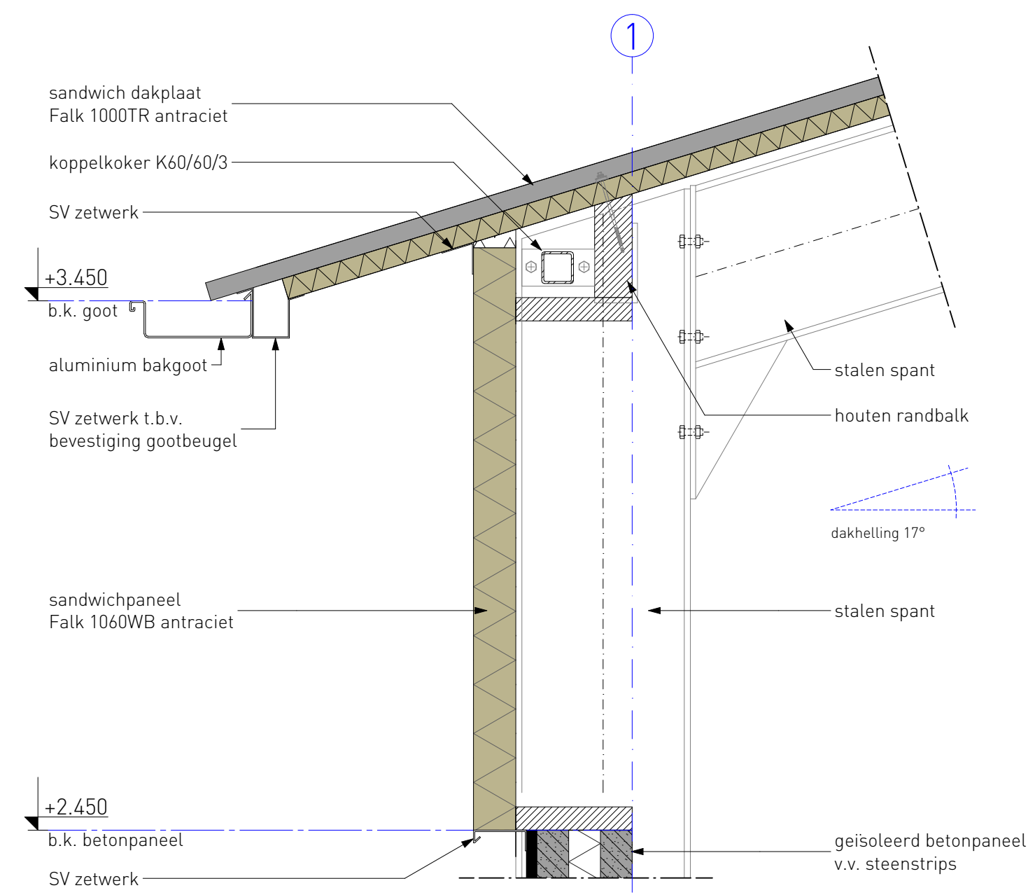
DETAIL 2 GOOT
