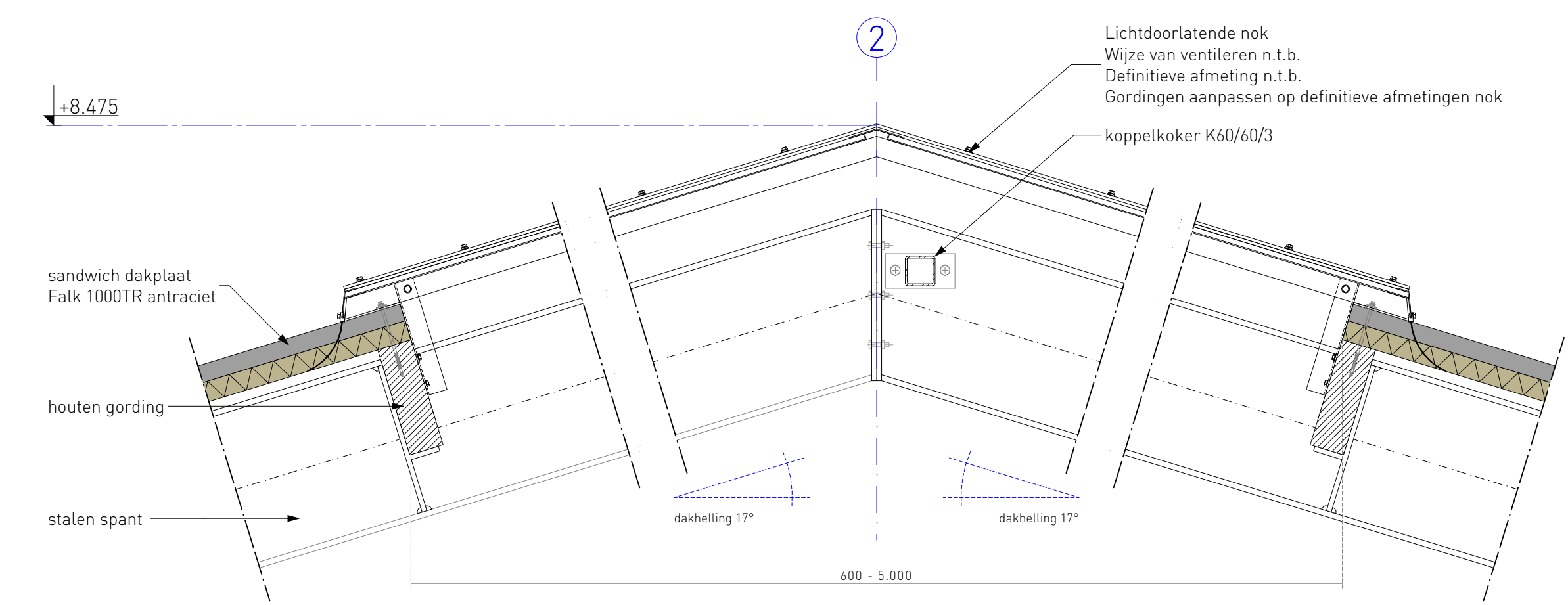
DETAIL 3 NOK
