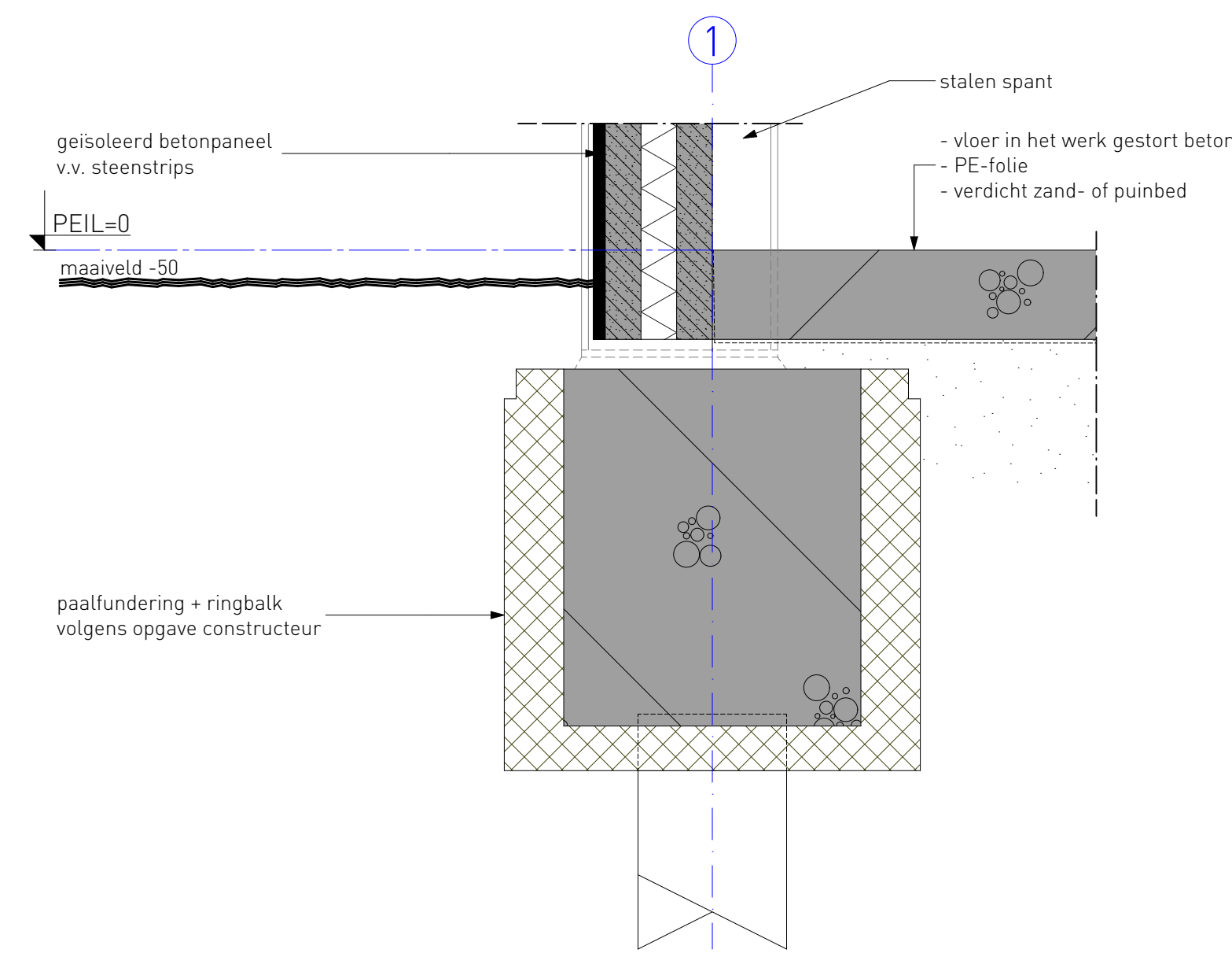
DETAIL 1 FUNDERING
