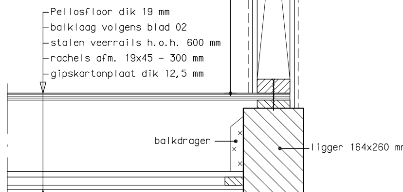
DETAIL C4c balustrade vide
