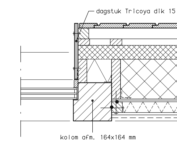
DETAIL C3g glas-hsb
