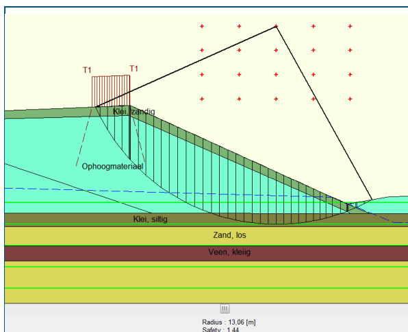
Glijcirkel dwp 4, Bishop (veiligheidsfactor 1,44)
