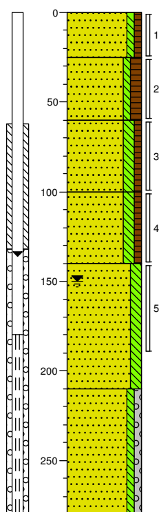
Boring: 03
