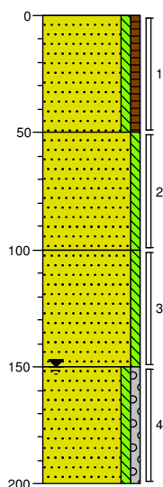
Boring: 05
