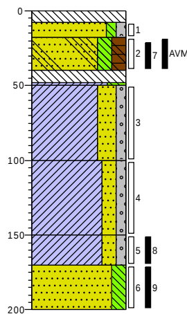
Boring: 14
