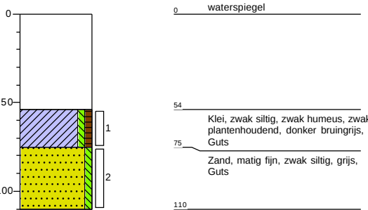
Boring: E02
