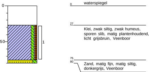
Boring: D09
