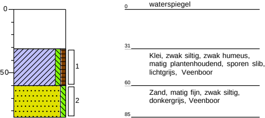
Boring: D05
