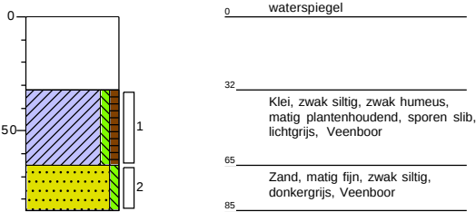
Boring: D06
