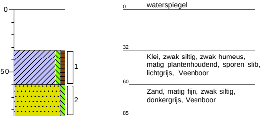
Boring: D08
