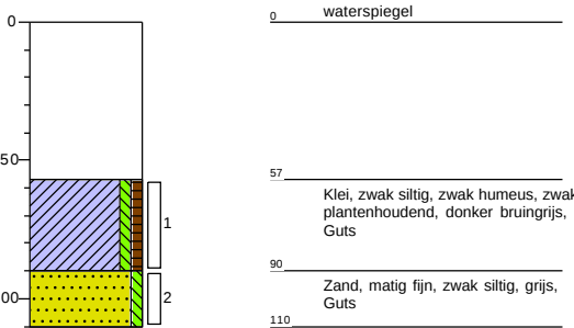
Boring: E01
