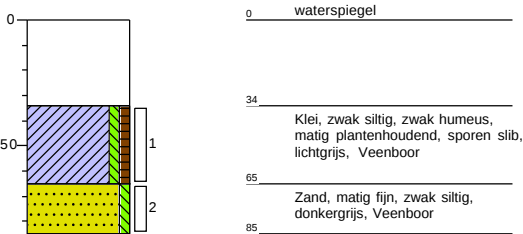
Boring: D07
