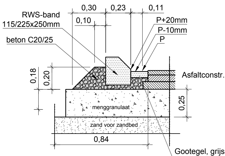
Detail RWS-band langs asfaltverharding schaal 1:20
