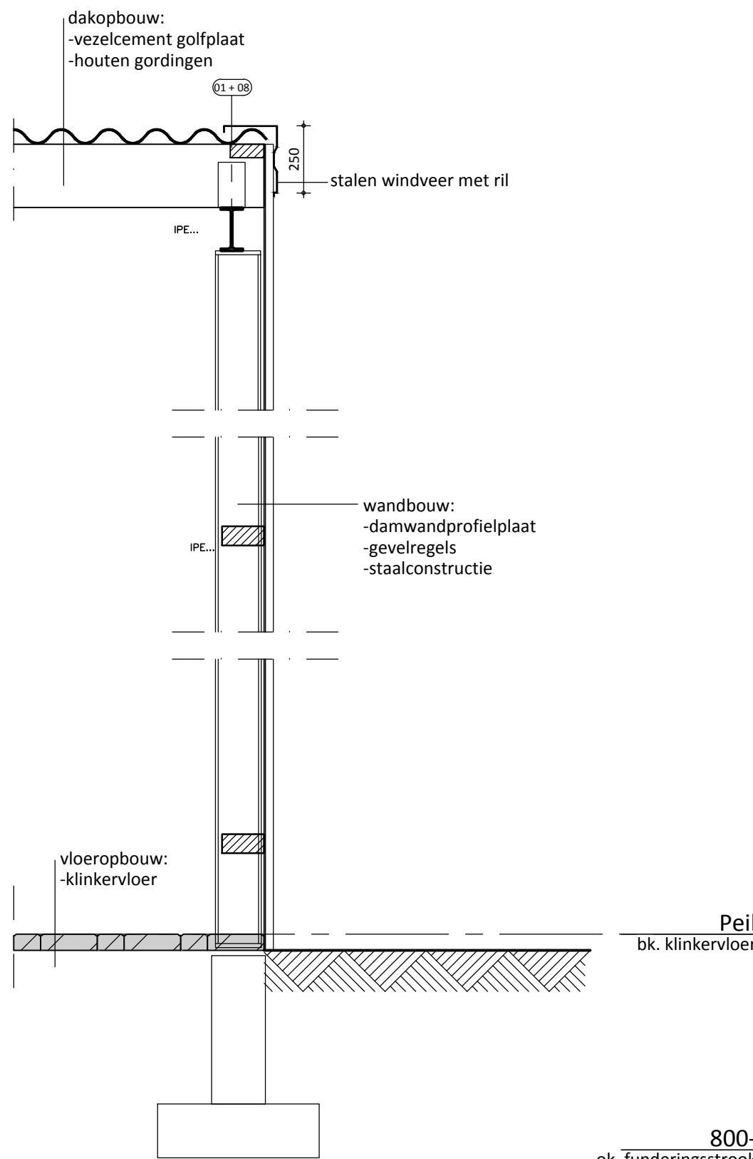
detail as 01 + 08
