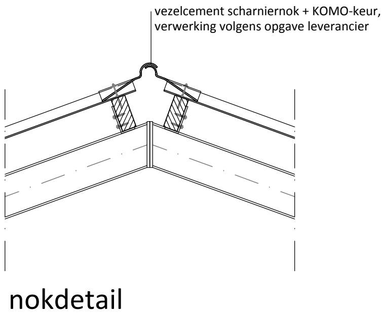
nokdetail
