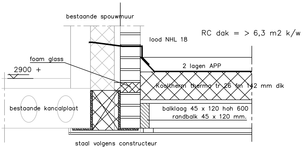
detail 3
