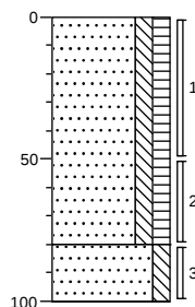
Boring: A04
