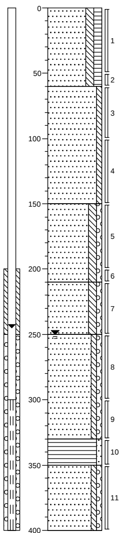
Boring: A01
