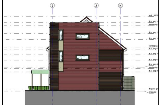
06. blok 6 - gevel as 39
