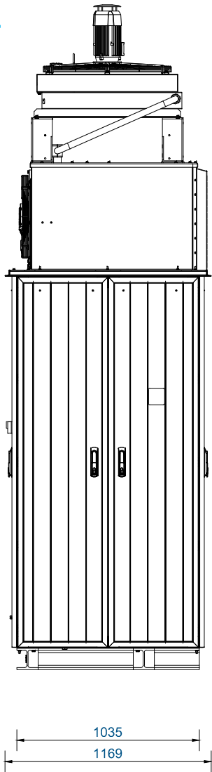
VIEW RIGHT
