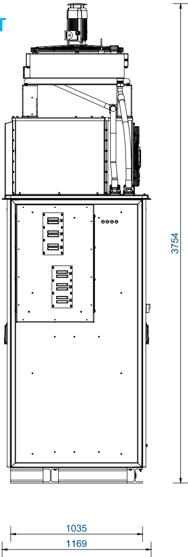
VIEW LEFT
