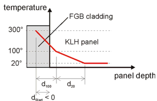
Figure 21: Temperature profiles for non cladded and cladded KLH® - CLT
